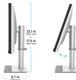
115mm Height Adjustment | Tilt -5~20°
